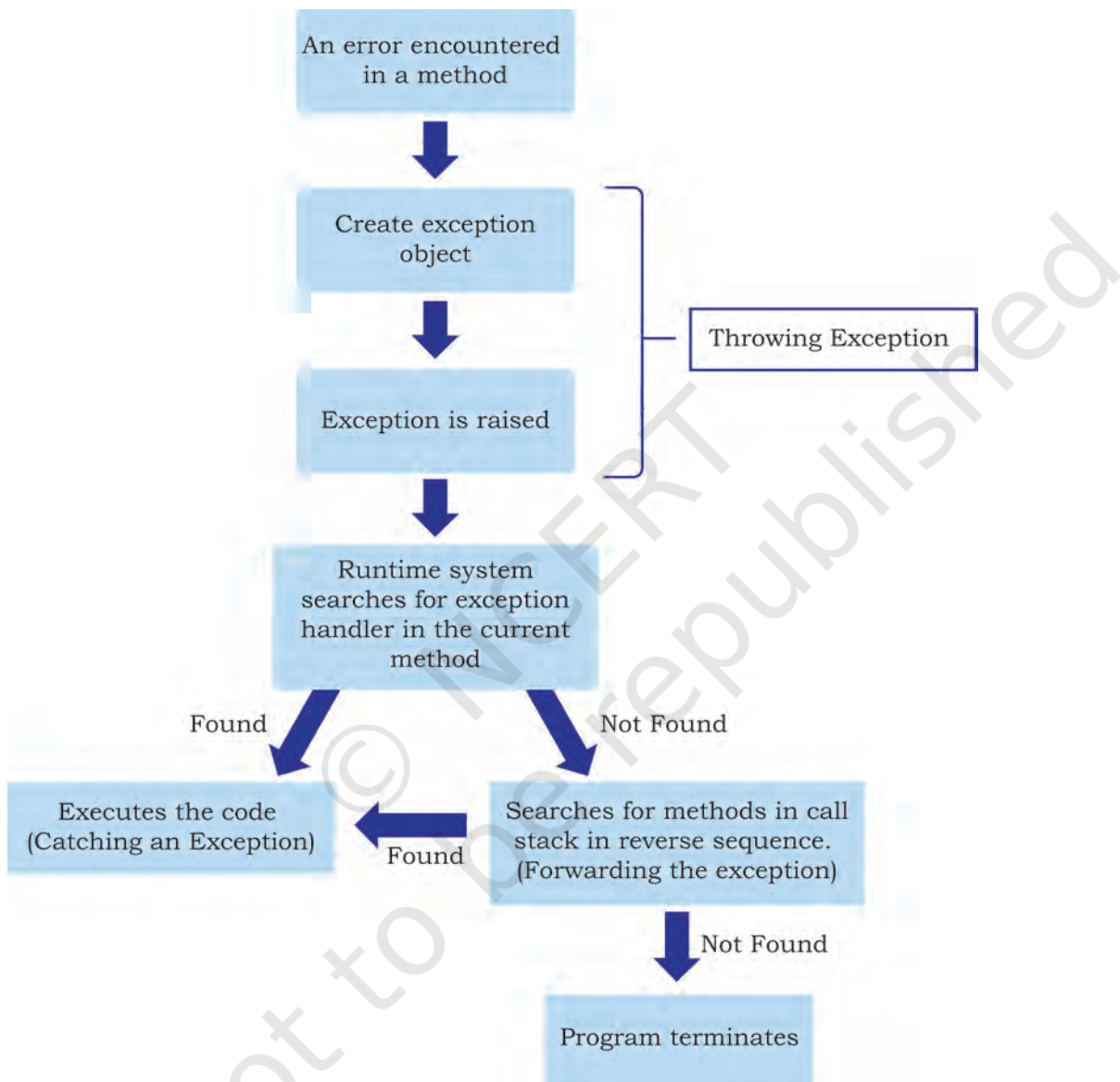
Figure 1.8: Steps of handling exception
