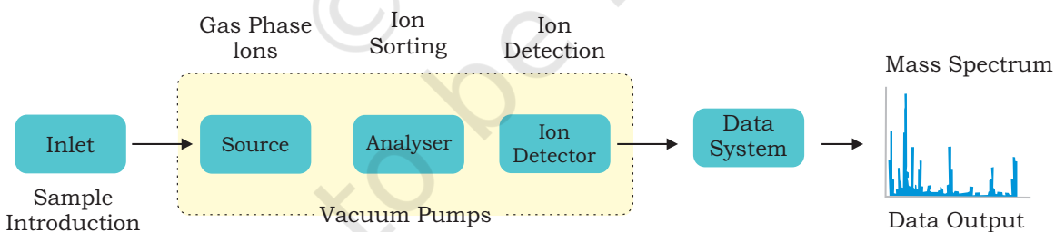
Fig. 12.14: Mass spectrometer
