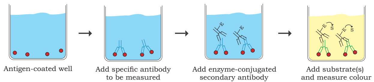
Fig. 12.6: Indirect ELISA
