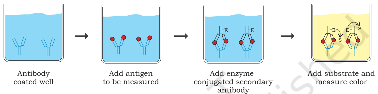
Fig. 12.7: Sandwich ELISA
