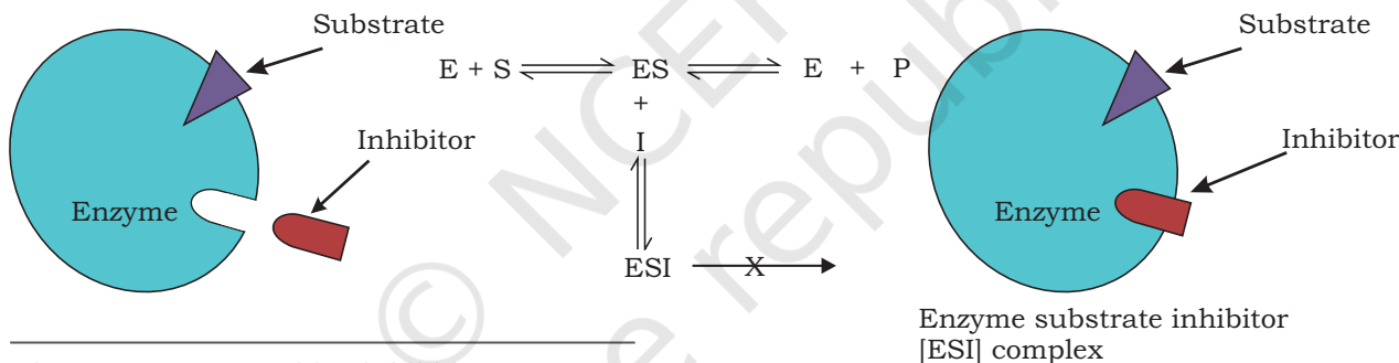
Fig. 4.11: Uncompetitive inhibition
