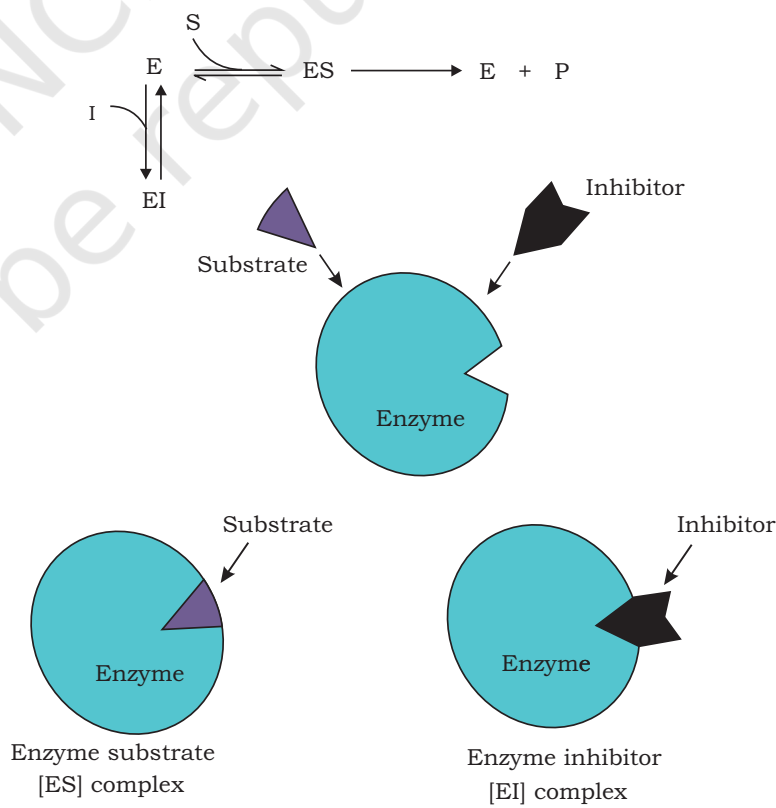
Fig. 4.7: Competitive inhibition
