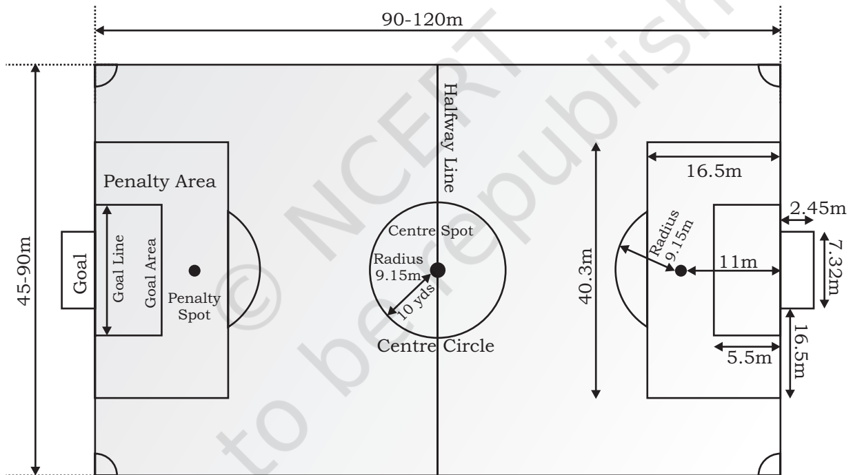
Fig. 6.16: Specifications of football ground
